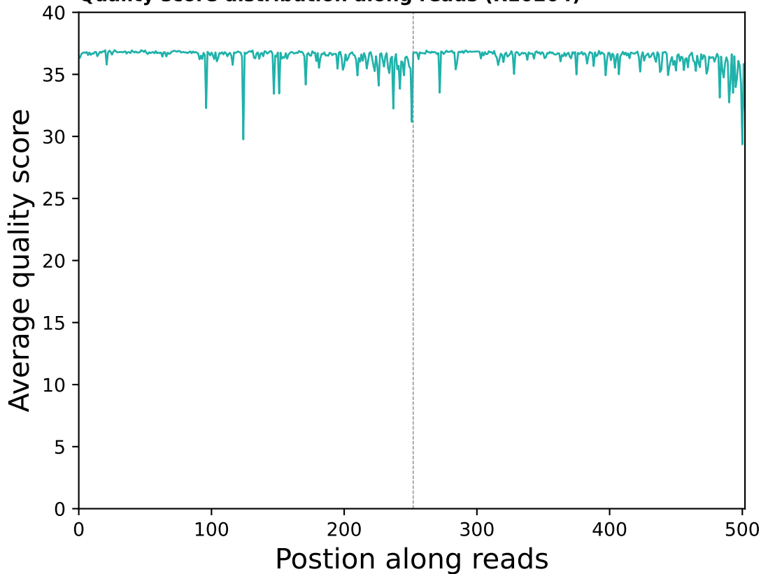
Quality score distribution along reads (R10204)
